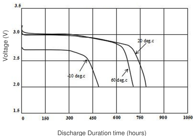
Discharge Characteristics; Discharge Load 15Kohm
